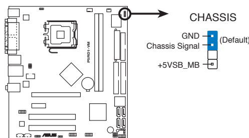
P5RD1-VM Chassis intrusion connector
