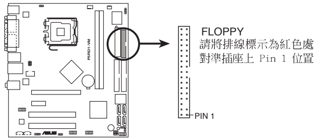
P5RD1-VM Floppy disk drive connector
