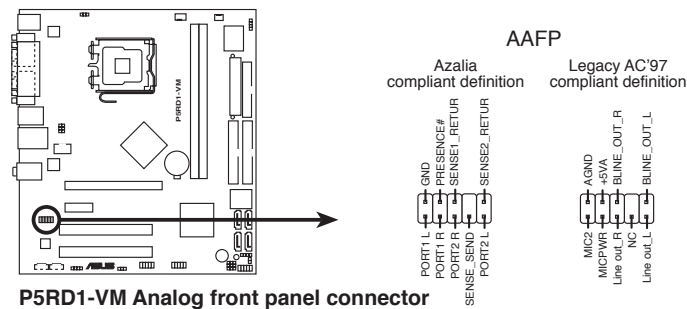
P5RD1-VM Analog front panel connector
