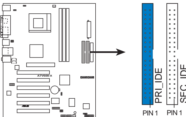
A7V600-X IDE Connectors
