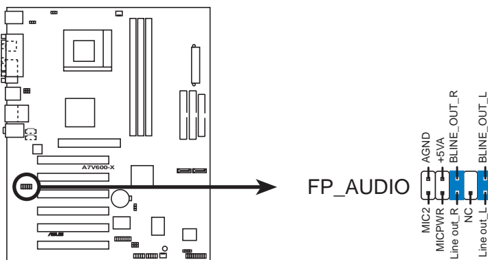
A7V600-X Front Panel Audio Connector
