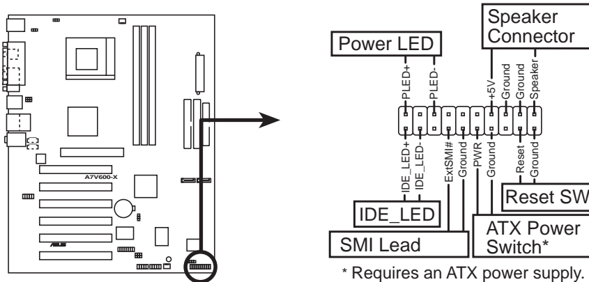
A7V600-X System Panel Connectors
